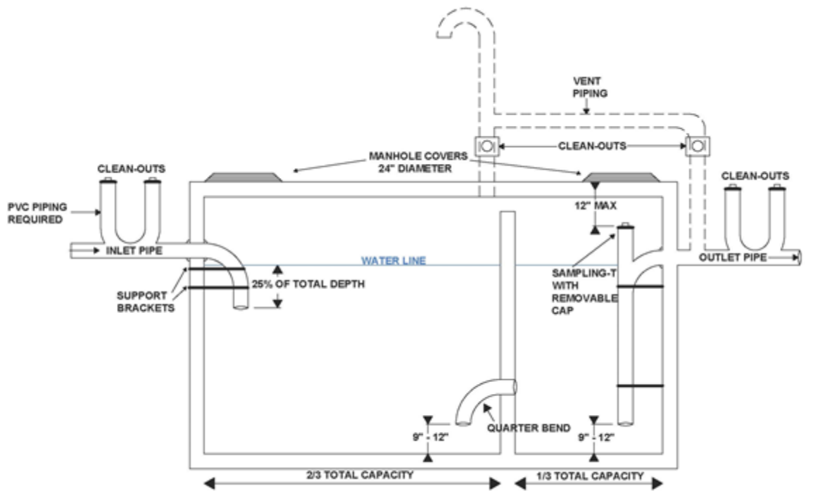
Figure 1: Gravity Grease Interceptor
